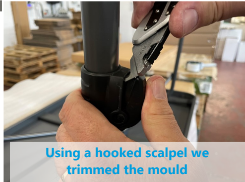
The plastic mould prevented the latch from being pressed in order to unlock the legs
